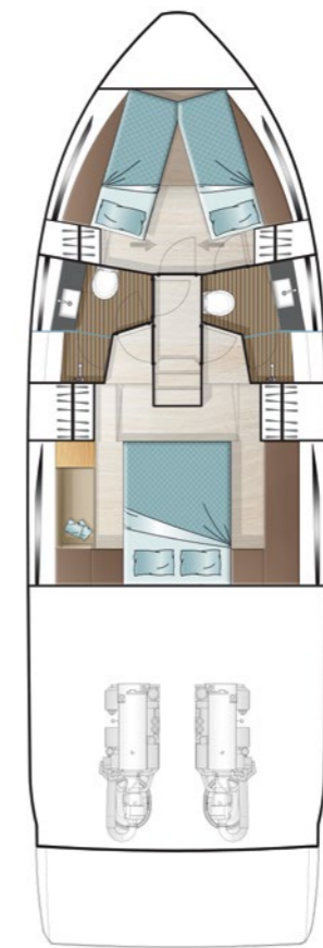
LOWER DECK
